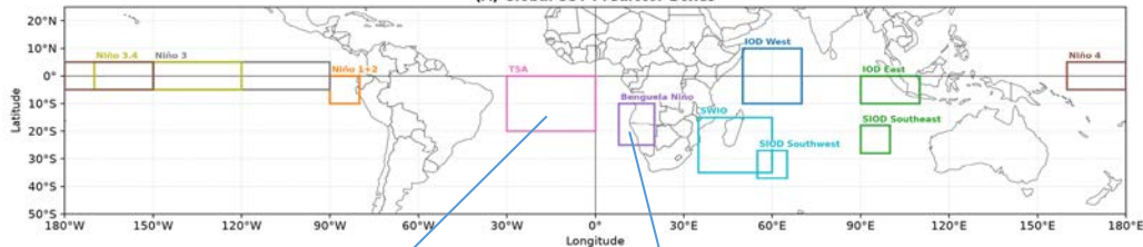
(A) Global SST Predictor Boxes
